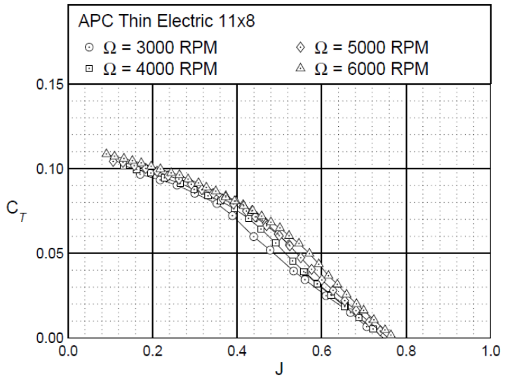
Figure 3- Typical coefficient of thrust vs. advance ratio plot [3]
