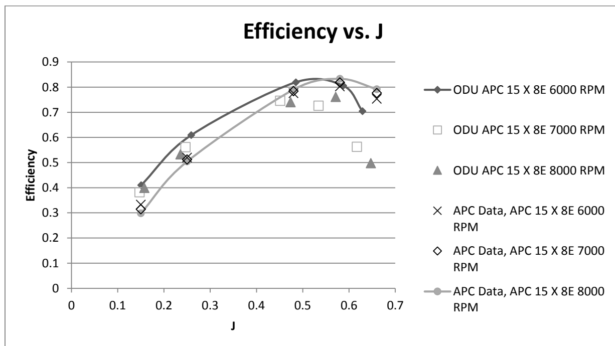
Figure 37- APC efficiency data compared to experimental results
