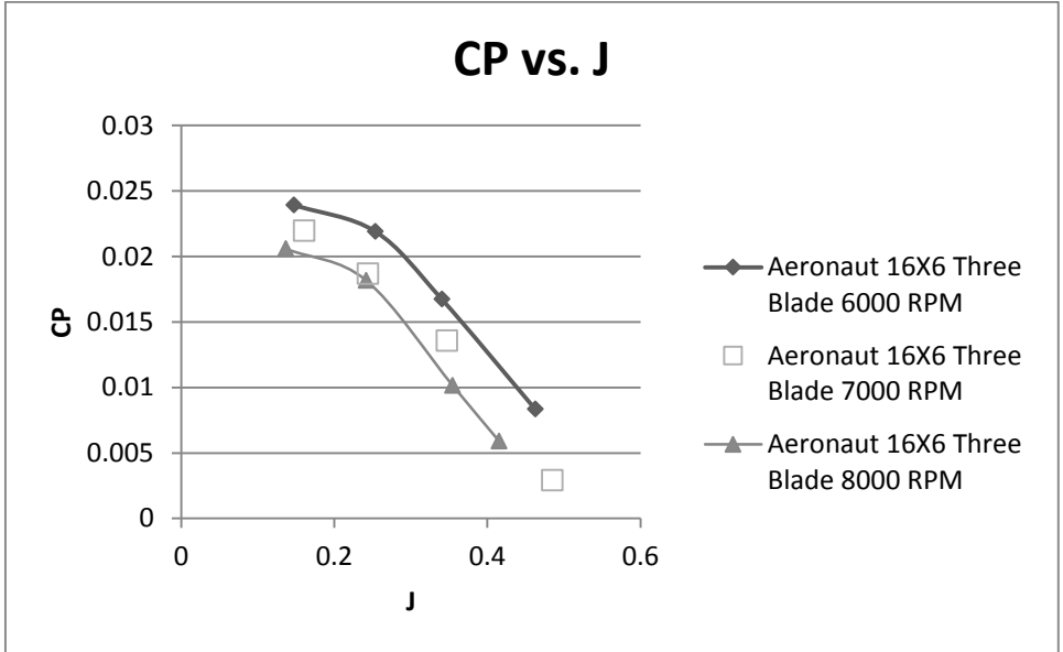
Figure 70- Aeronaut 16×6 three blade coefficient of power vs. advance ratio results
