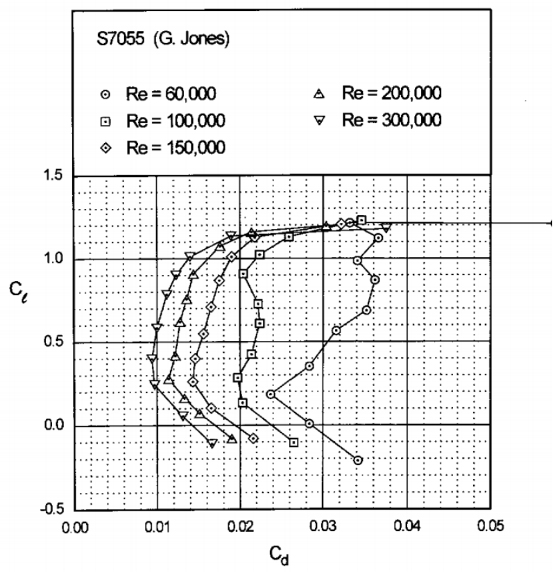
Figure 6- Low-Speed Airfoil Data shows increased performance with increased Reynolds number [5]
