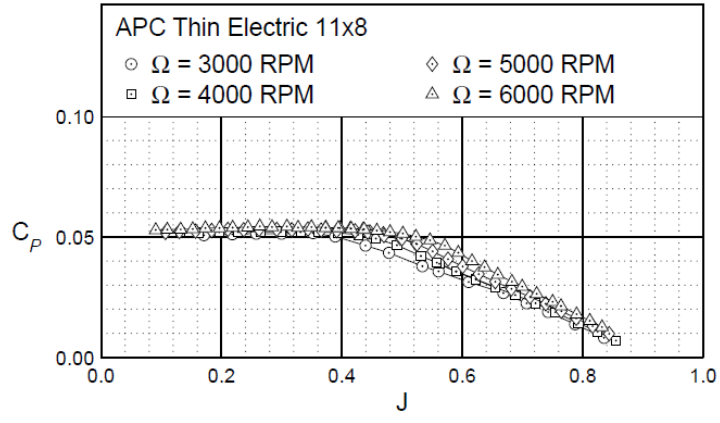
Figure 4- Typical coefficient of power vs. advance ratio [3]
