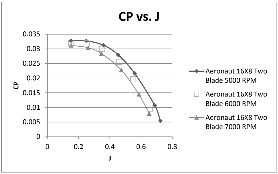
Figure 63- Aeronaut 16x8 two blade coefficient of power vs. advance ratio
