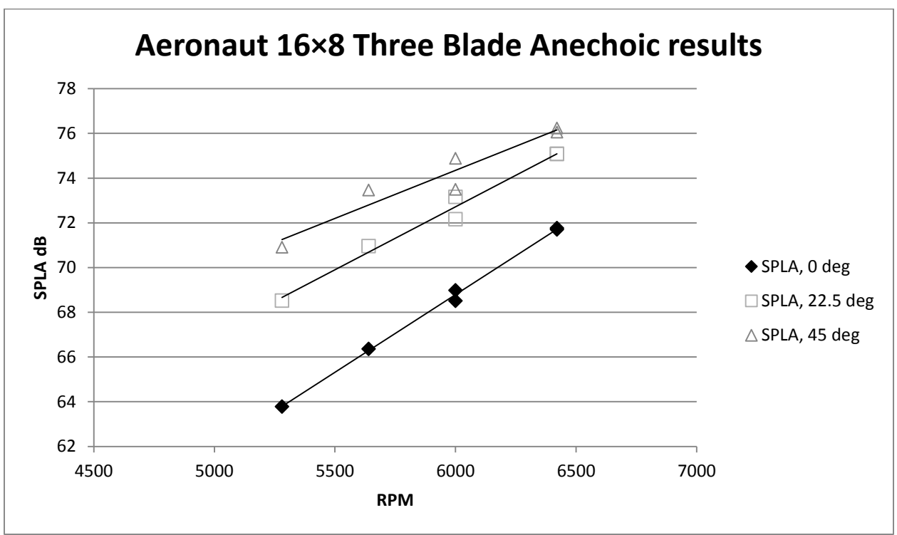
Figure 54- Anechoic chamber Aeronaut 16x8 three blade acoustic data at varying angles
