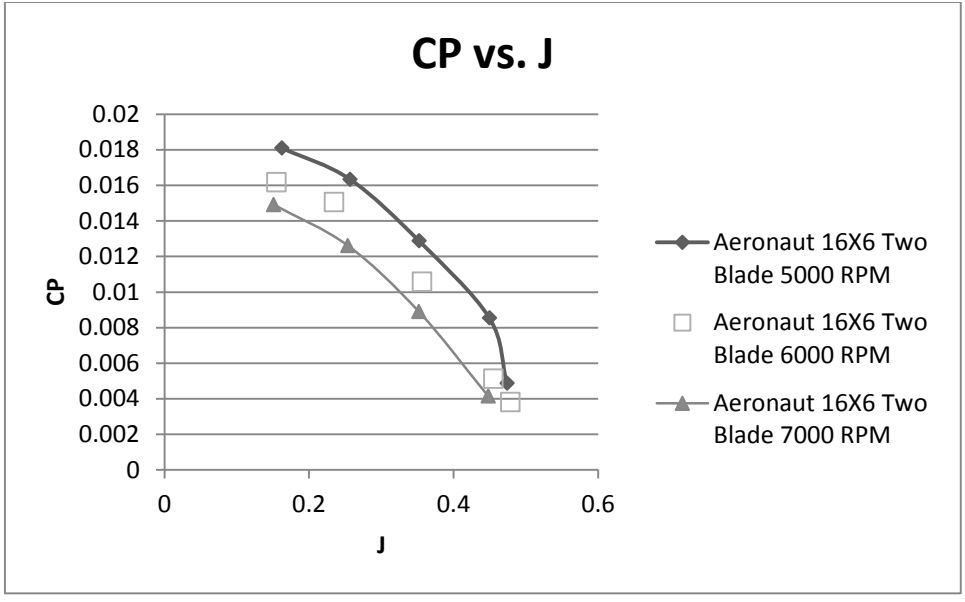
Figure 62- Aeronaut 16x6 two blade coefficient of power vs. advance ratio
